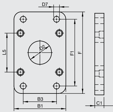
FM FOOT MOUNTING
