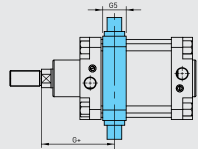
CTM CENTRAL TRUNNION MOUNTING
