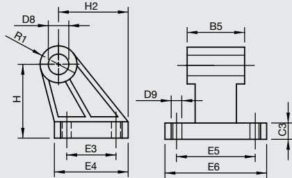
CFM CLEVIS FOOT MOUNTING
