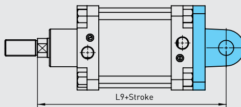
SFWCFM SWIVEL FLANGE WITH CLEVIS FOOT MOUNTING
