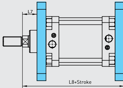
FLM FLANGE MOUNTING
