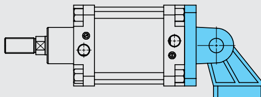
SFWCFM SWIVEL FLANGE WITH CLEVIS FOOT MOUNTING
